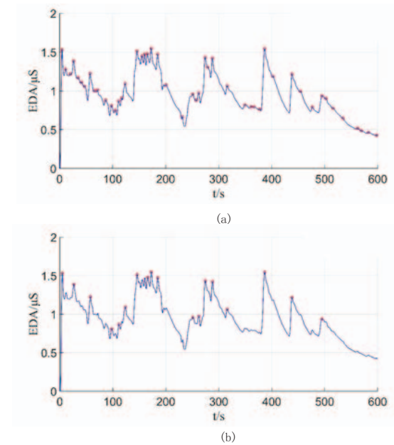
Fig8. AI EDA algorithm with localization strategy (a) before data preprocessing;(b) after data preprocessing.
