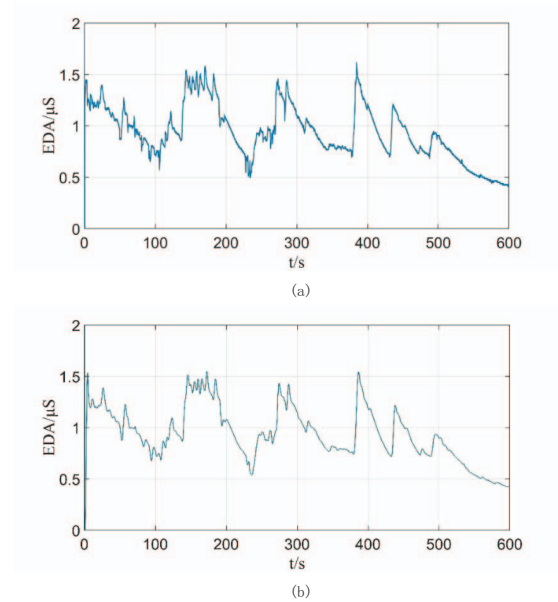
Fig6. Butterworth filters (a) before data preprocessing; (b) after data preprocessing.
